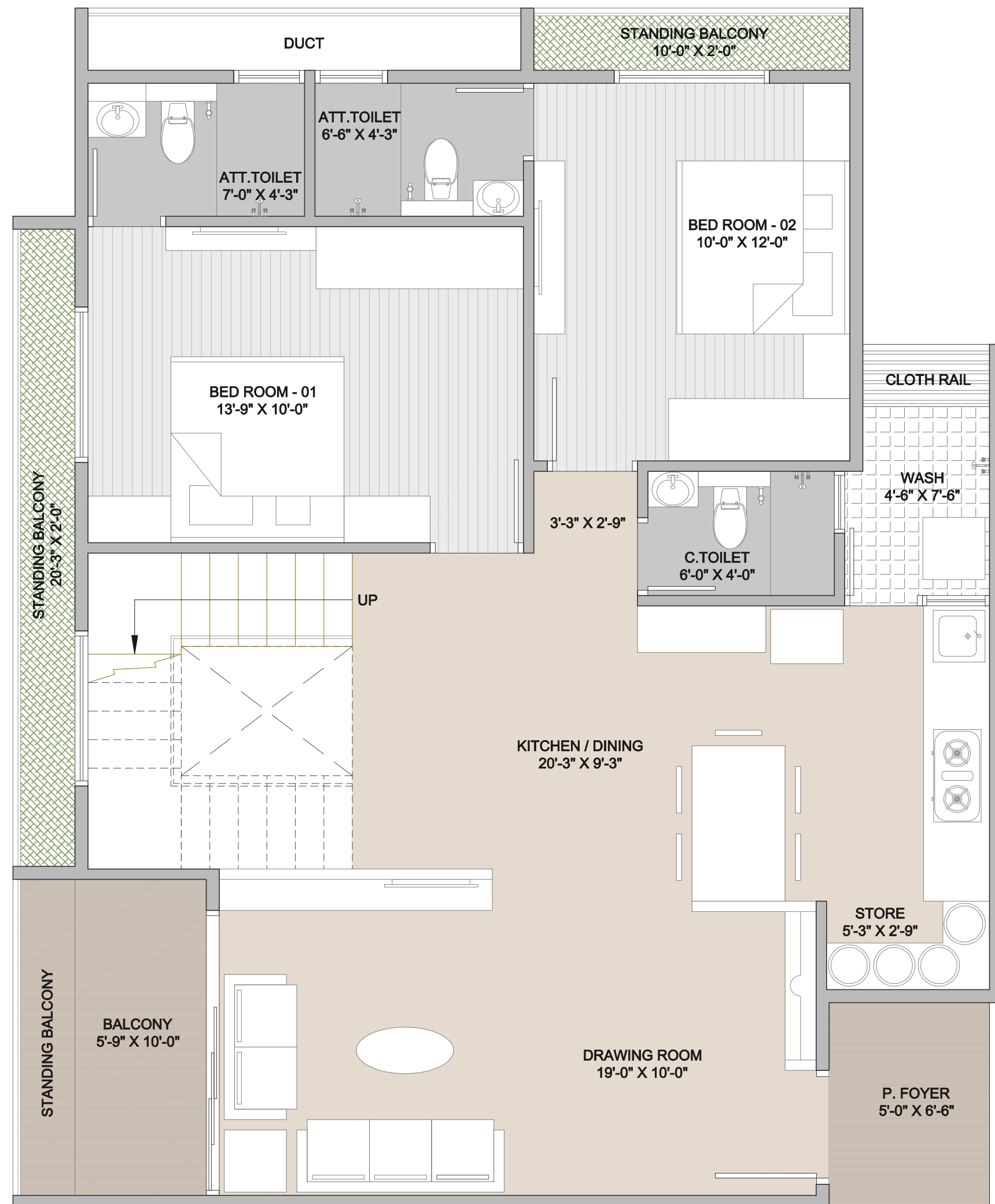
13TH FLOOR LAYOUT
